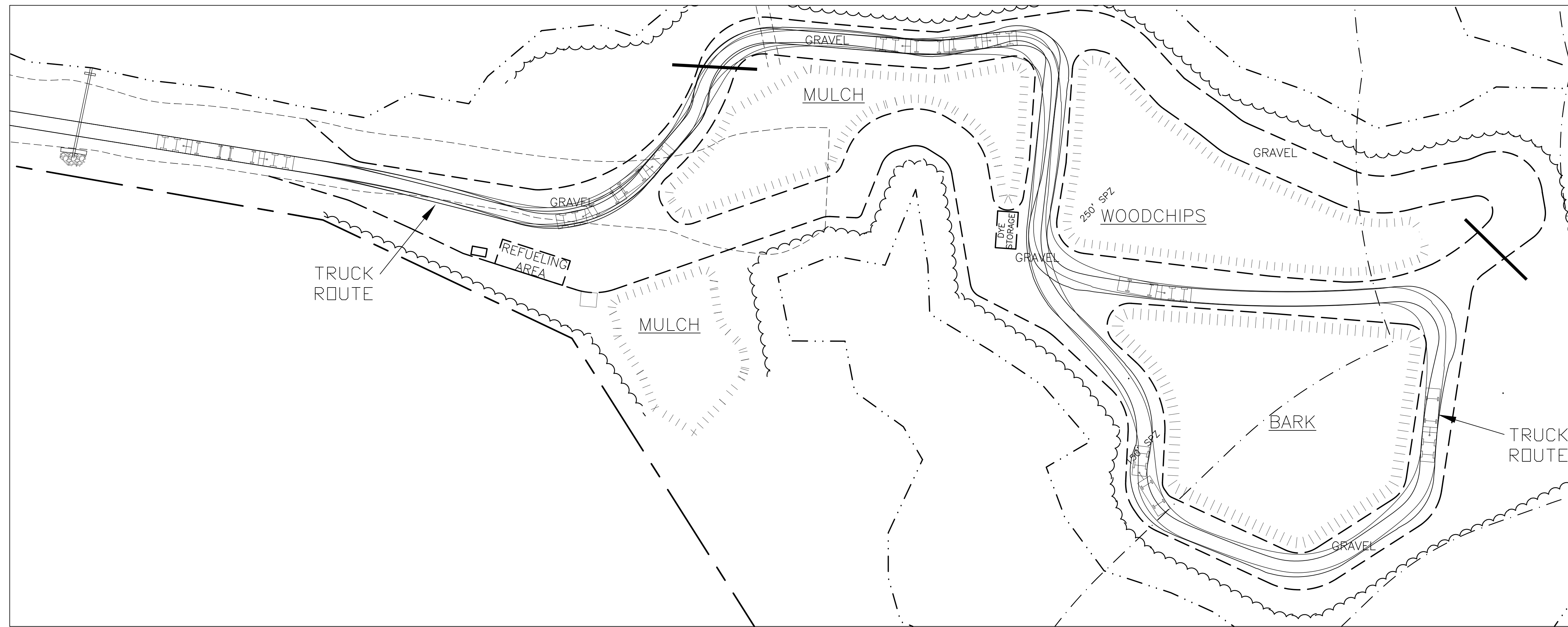
WB-50 TRUCK MANEUVERING
